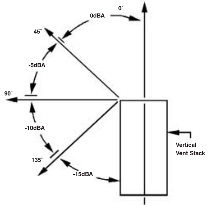
Figure 5 Directivity Index
