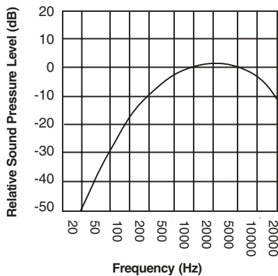
Figure 1 IEC Standard A-Weighting Curve for Sound Level Meters
