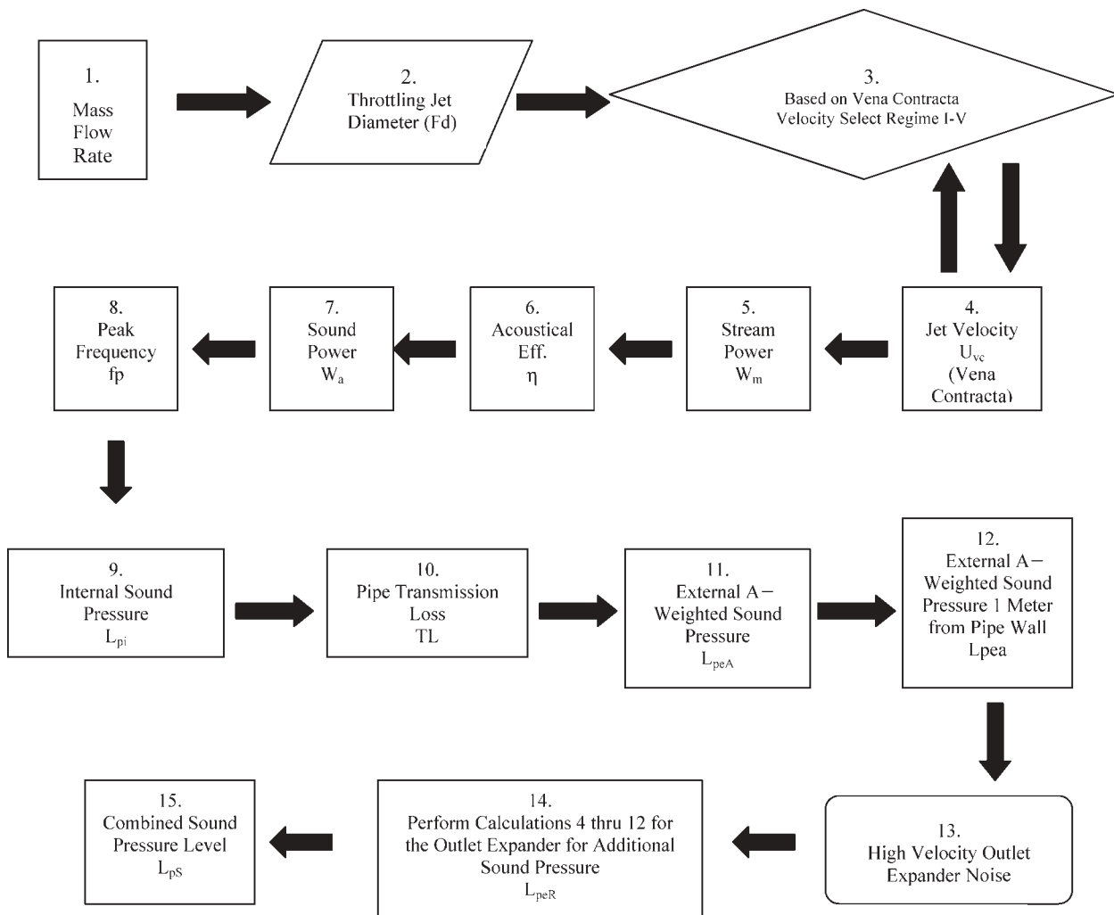
Control Valve Aerodynamic Noise Prediction Flow Chart
