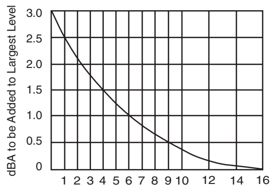
Figure 4 Decibel Difference Between Two Sound Levels dBA
