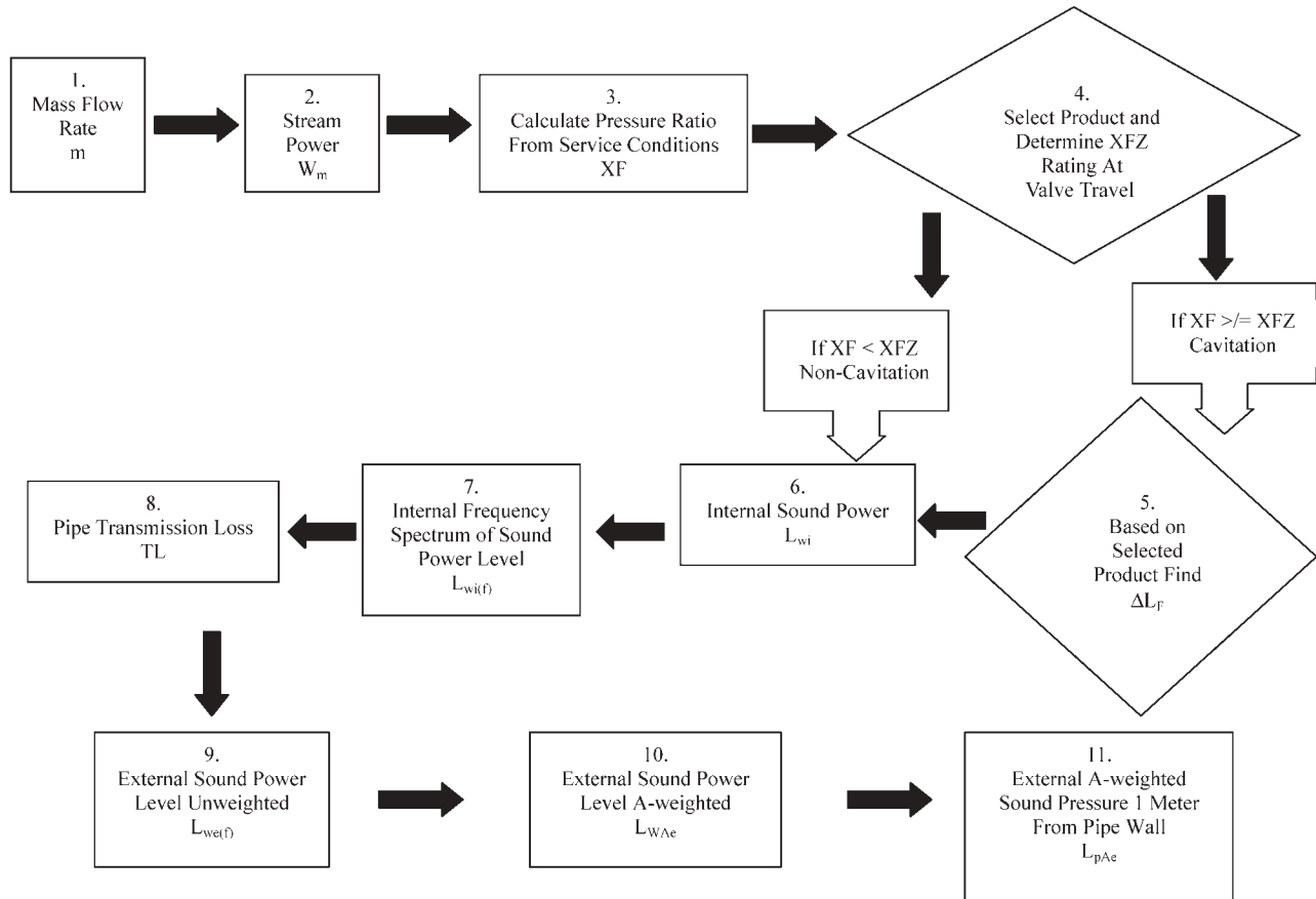
Hydrodynamic Noise Prediction Flow Chart
